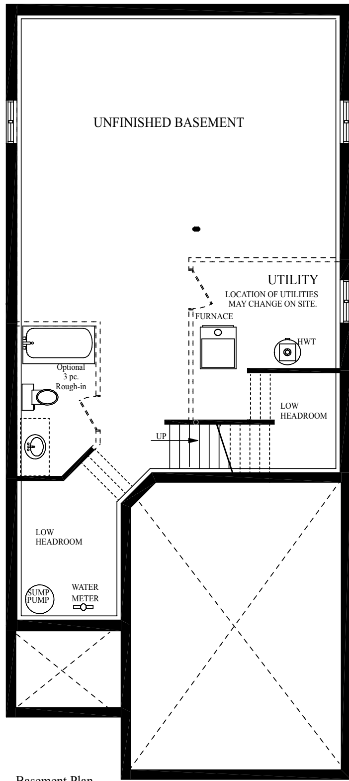
Basement Plan
