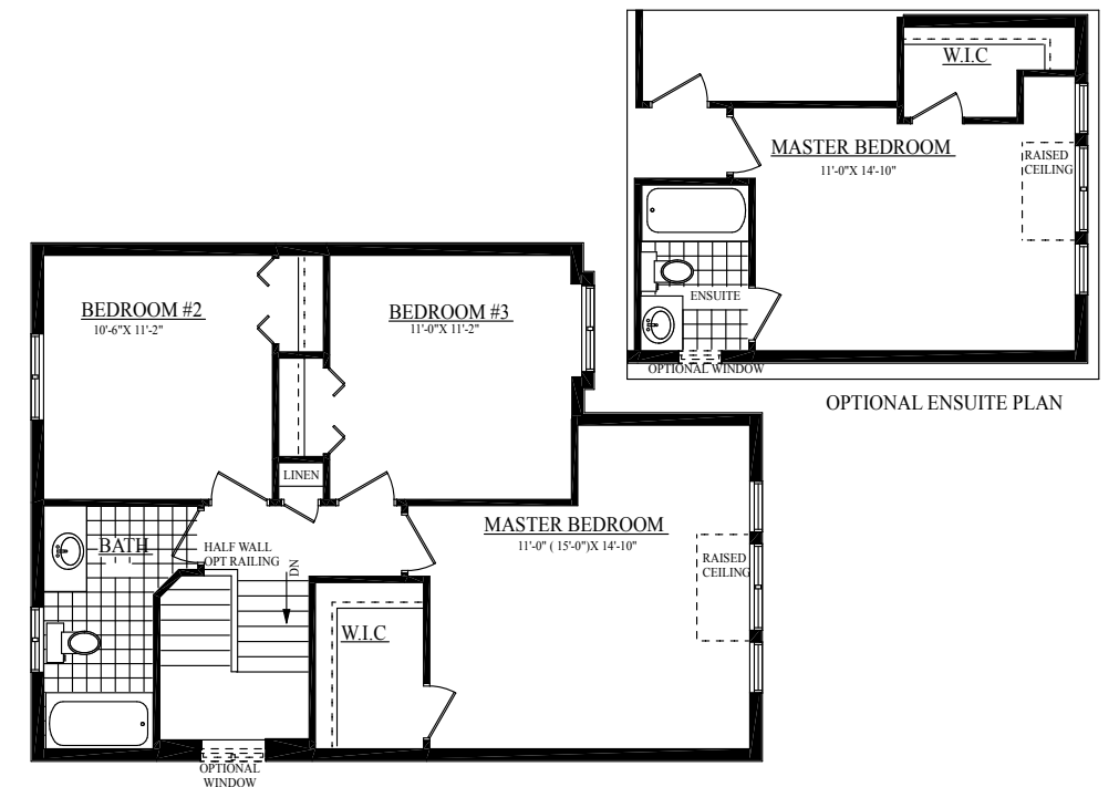
SECOND FLOOR PLAN C
