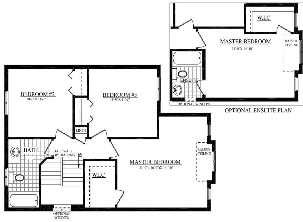
SECOND FLOOR PLAN B
