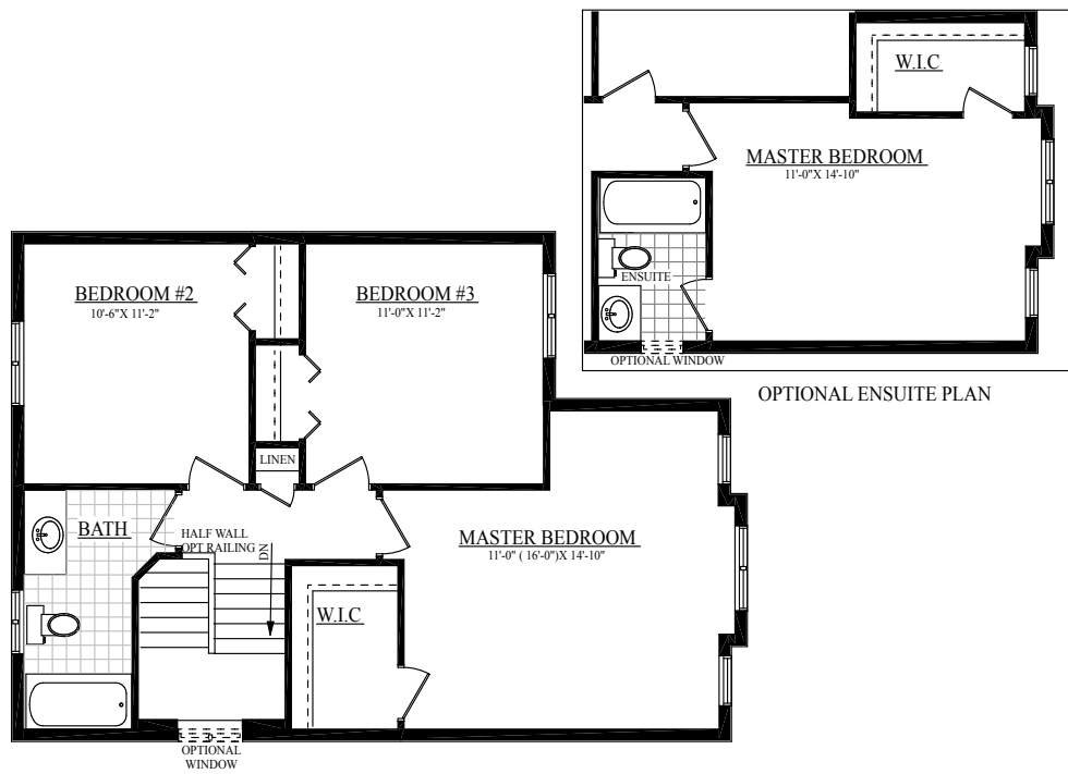
SECOND FLOOR PLAN A
