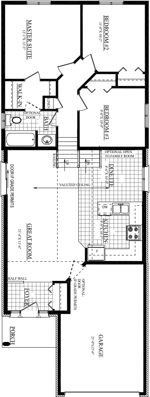
MAIN FLOOR PLAN C
