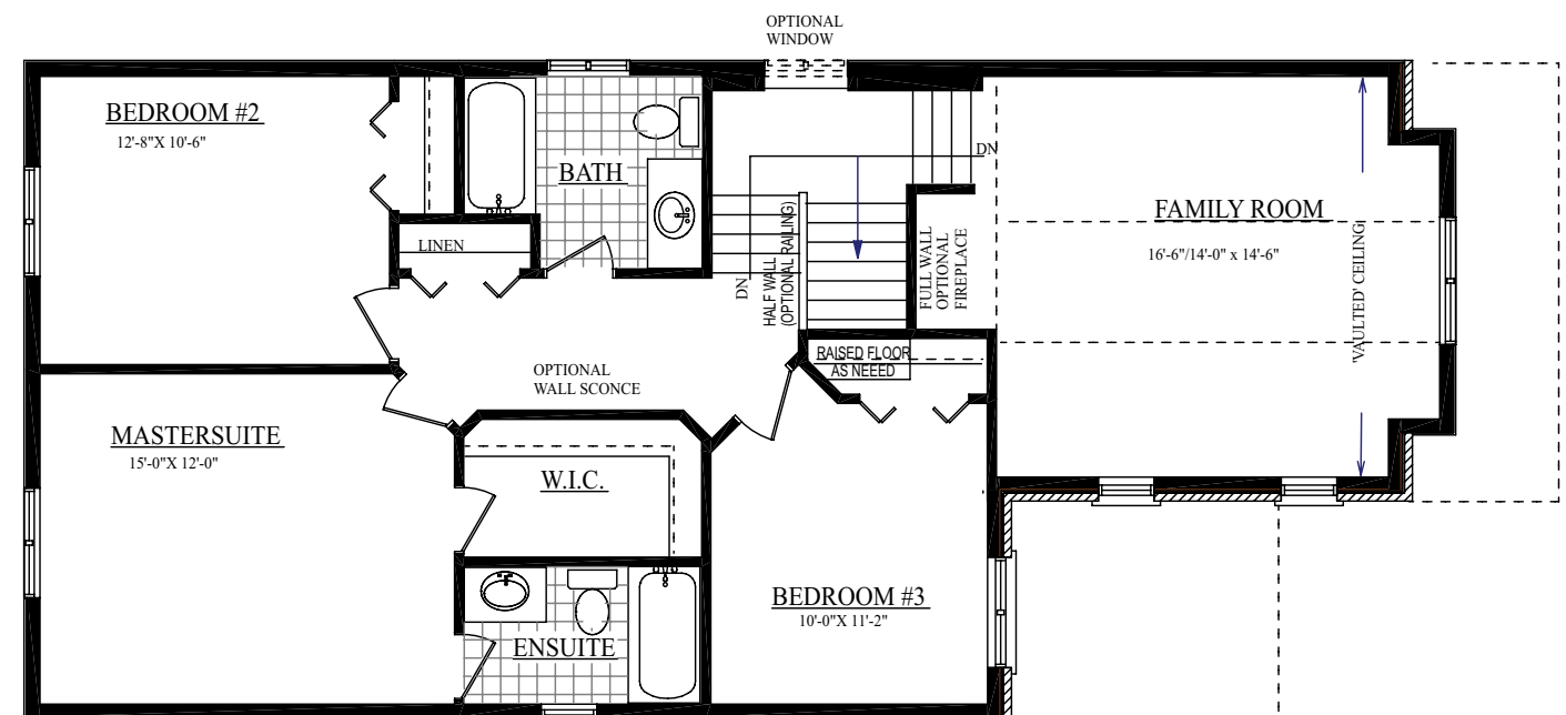
SECOND FLOOR PLAN B
