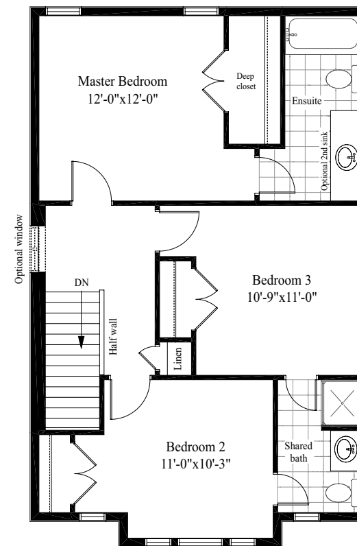
SECOND FLOOR ELEVATION A OPTIONAL ENSUITE
