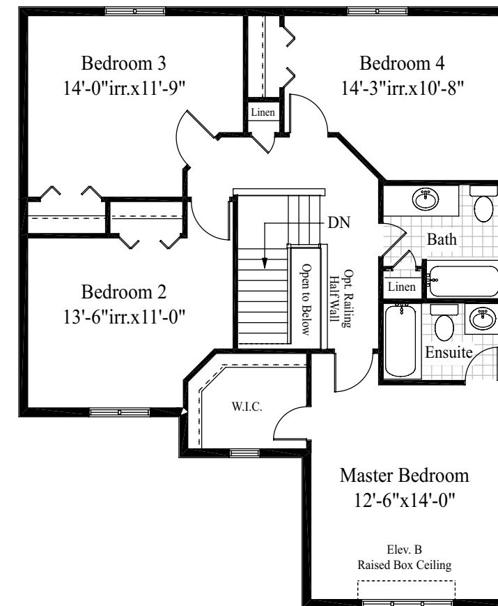
SECOND FLOOR PLAN with OPT. LUXURY ENSUITE
