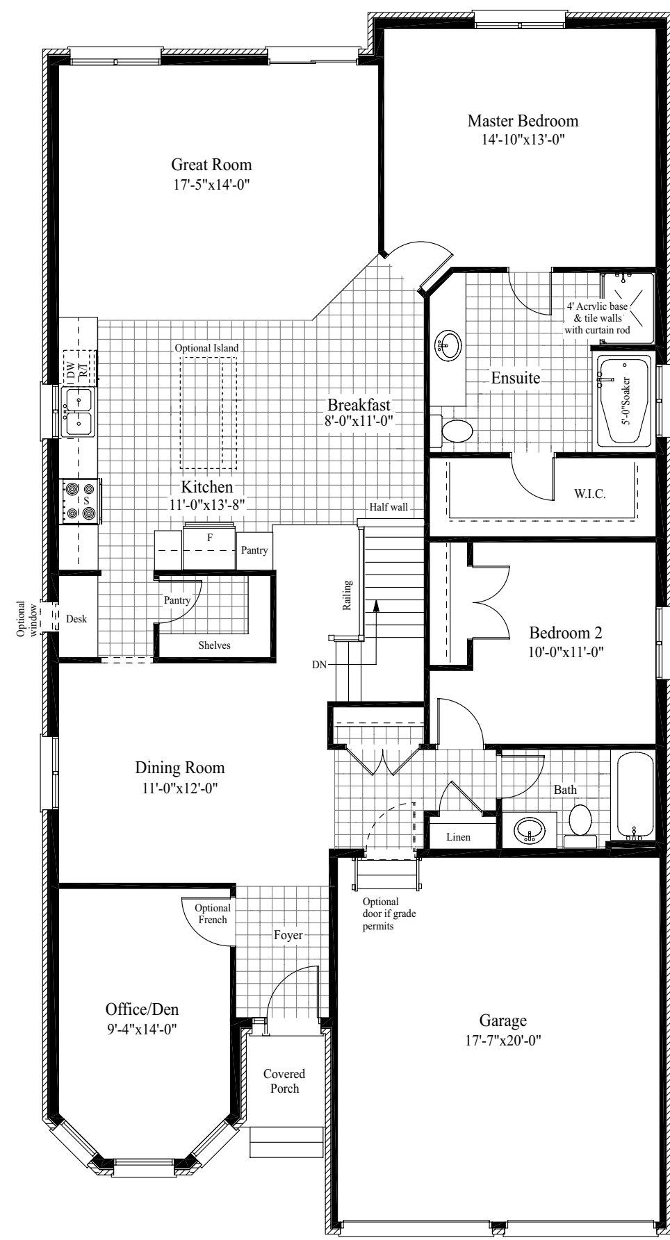
FIRST FLOOR PLAN - ELEVATION B
